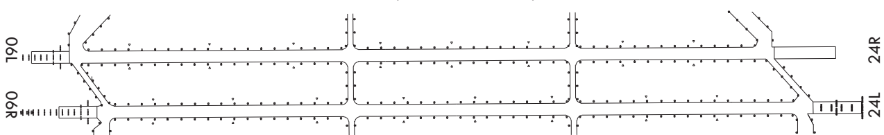
LIGHTING AIDS RWY 06L/24R AND 06R/24L AND EXIT TWY
